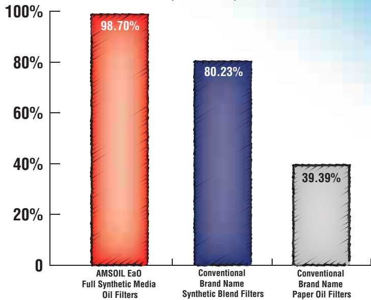
Filter Efficiency @ 15 Micron per ISO 4548-12
